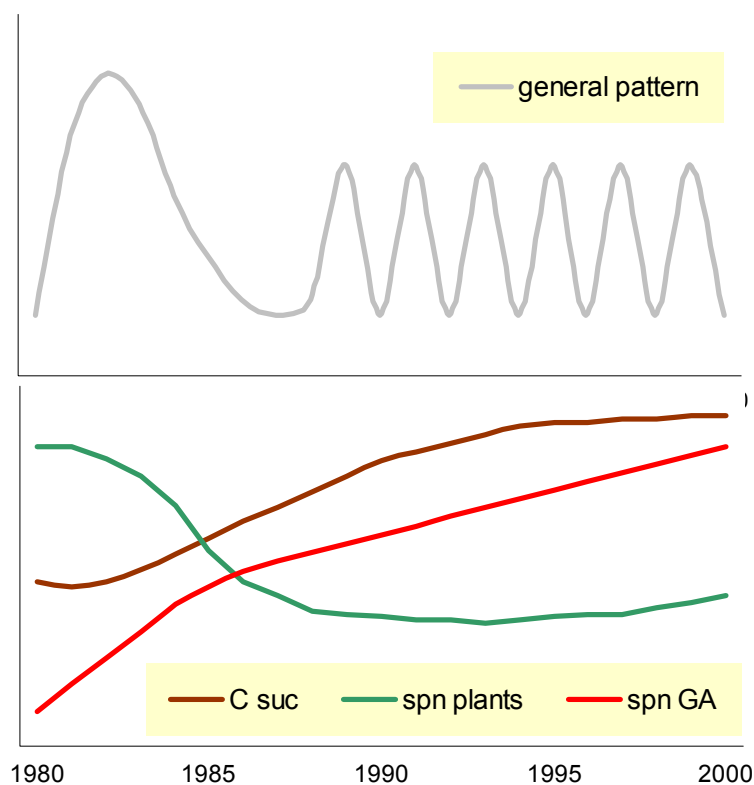
Fig. 2: Generalized trends for soil mesofauna abundances (top) and C-content of soil, as well as for species numbers of plants (spn plants) and Gamasina (spn GA)
